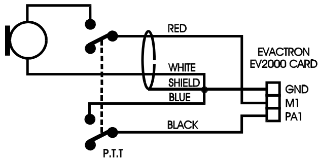
ALTRONICS C0335 MIC CONNECTIONS
