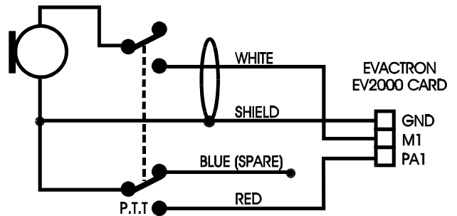
ALTRONICS C0333 MIC CONNECTIONS
